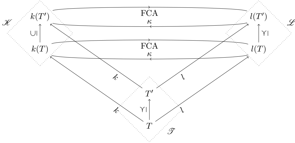
Figure 7: Relations between \mathcal{T} , \mathcal{K} and \mathcal{L} .
