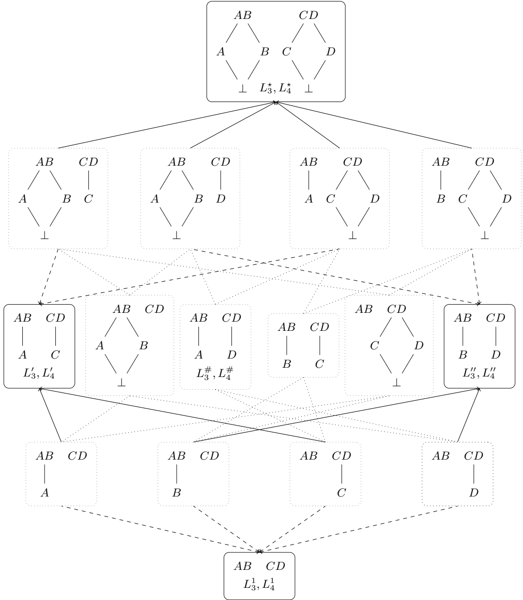
Figure 9: All the families of lattices belonging to [\text{lfp}(EF^*) \text{ gfp}(PQ^*)] in the example of Section 3.2. Those in \text{fp}(EF^*) \cap \text{fp}(PQ^*) are within solid boxes. As usual, only direct edges are displayed. Solid arrows show direct application of EF^* and dashed arrows show direct application of PQ^* . Dotted arrows are order relations not corresponding to EF^* or PQ^* applications.
