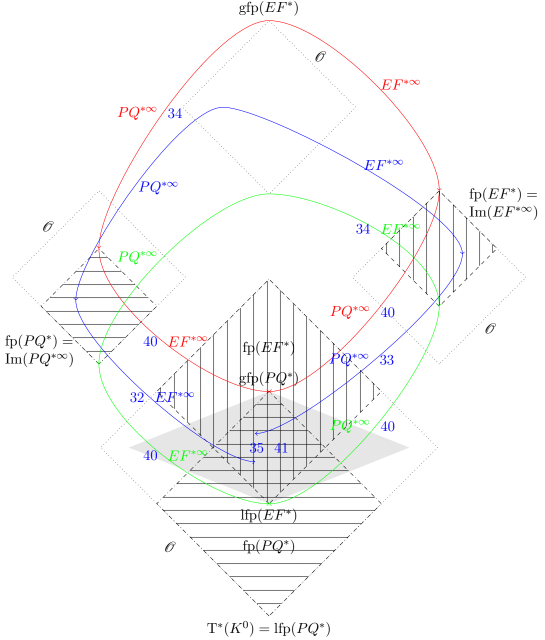
Figure 8: Illustration of Properties 32, 33, 35, 34, 36, 40 and 41. The figure displays four times \mathcal{O} and the images of \text{gfp}(EF^*) (red), a random family of context-lattice pairs (blue) and \text{lfp}(PQ^*) = T^*(K^0) (green) through PQ^{*\infty} (left) and EF^{*\infty} (right). \text{fp}(EF^*) is drawn in vertical lines; \text{fp}(PQ^*) in horizontal lines and the grey area depicts the interval [\text{lfp}(EF^*), \text{gfp}(PQ^*)] .
