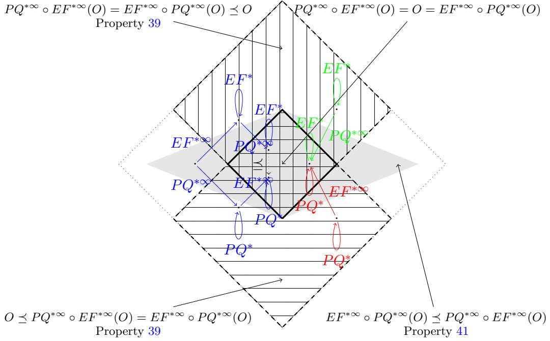
Figure 10: Illustration of the position of PQ^{*\infty} \circ EF^{*\infty}(O) and EF^{*\infty} \circ PQ^{*\infty}(O) depending on O 's origin (in dotted, \mathcal{O} , in dashed \text{fp}(EF^*) \cup \text{fp}(PQ^*) , in plain \text{fp}(EF^*) \cap \text{fp}(PQ^*) ). Colours correspond to that of Figure 8: green starting from \text{fp}(EF^*) , red starting from \text{fp}(PQ^*) , blue starting outside of them.
