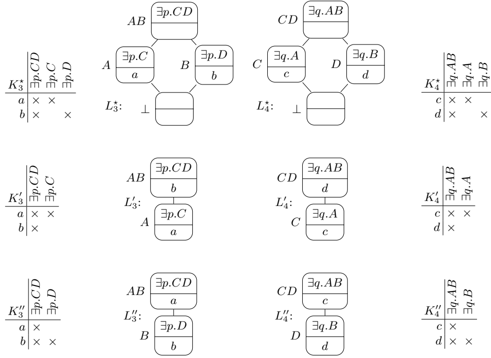
Figure 5: Alternative pairs of concept lattices covering the contexts of Figure 4.
