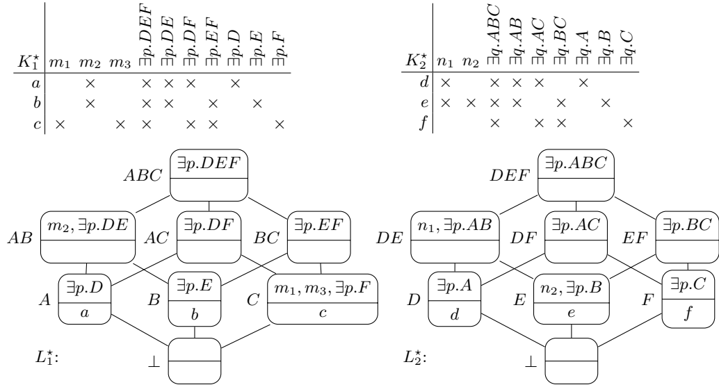
Figure 2: Alternative concept lattices for the example of Section 3.1 ( \star is simply a way to identify these objects).
